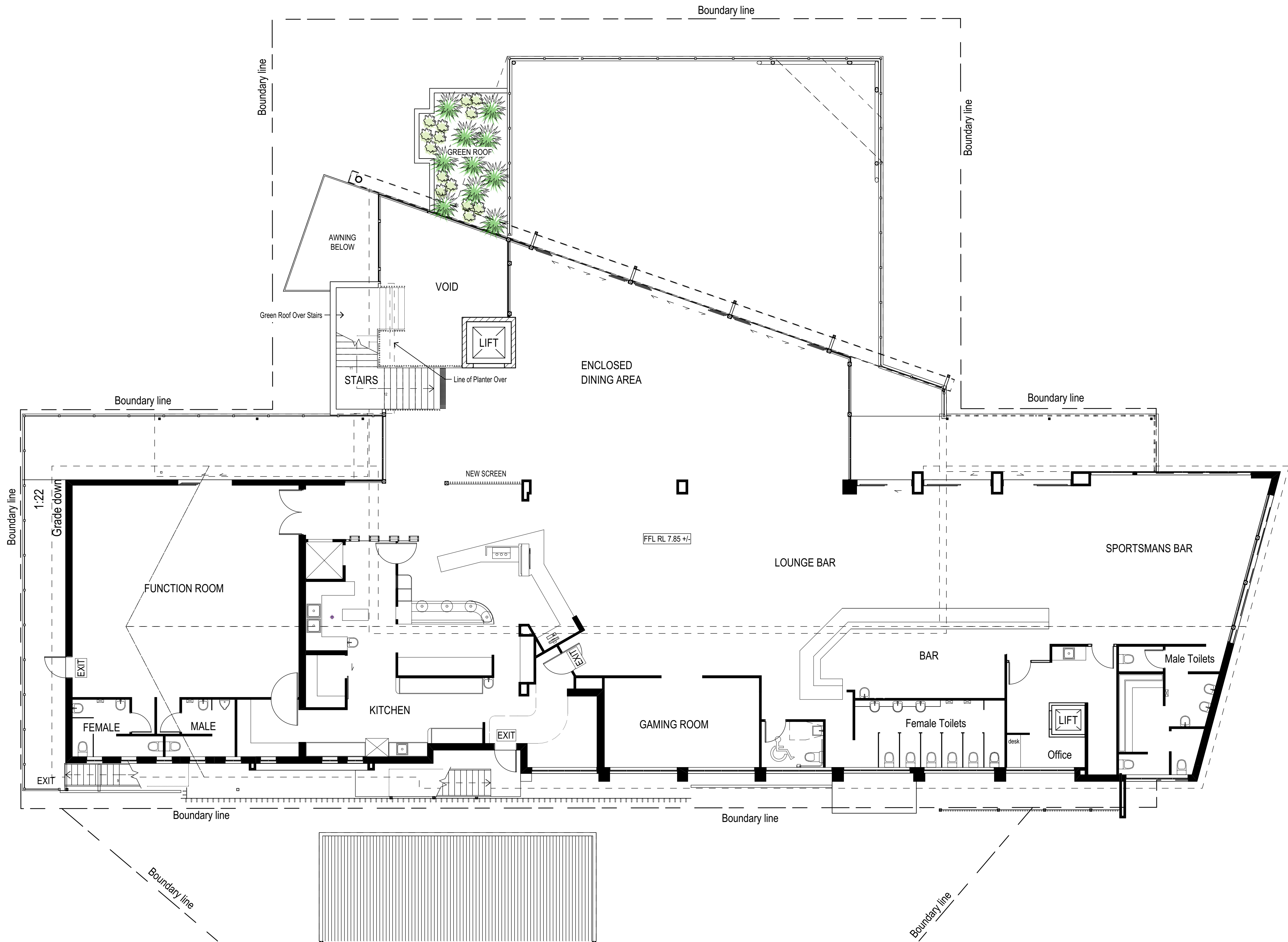
1 PROPOSED FIRST FLOOR PLAN Scale - 1:100
