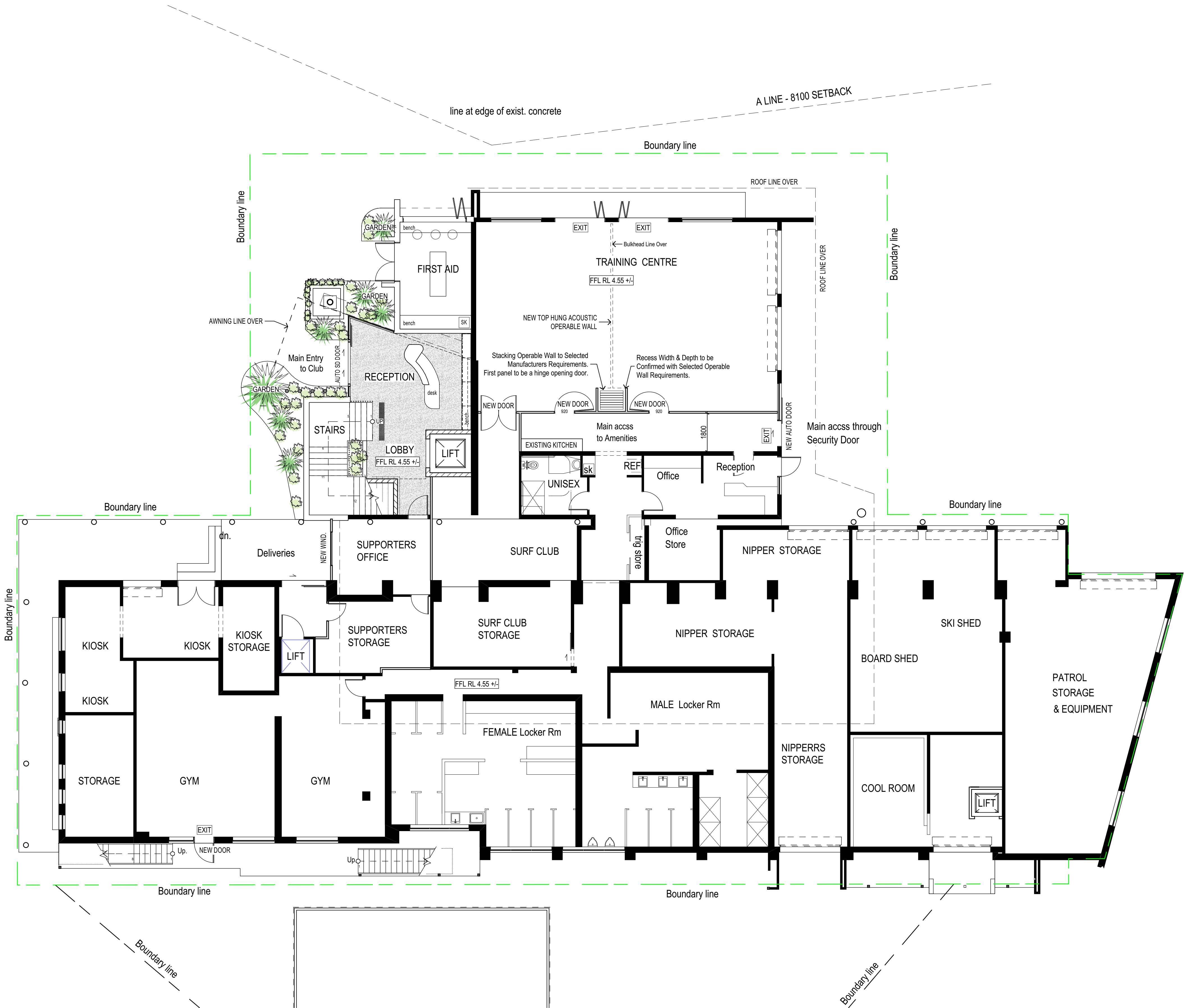
1 PROPOSED GROUND FLOOR PLAN Scale - 1:100 - @A1
